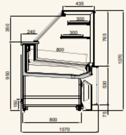
VETRINA PASTICCERIA NEUTRA NON-REFRIGERATED PASTRY SHOWCASE VITRINE NON RÉFRIGÉRÉE PATISSERIE VITRINE KONDITOREIWAREN NEUTRAL
